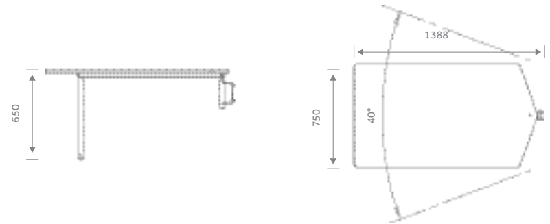
Dimensions (mm)
